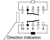
2-coil latching
